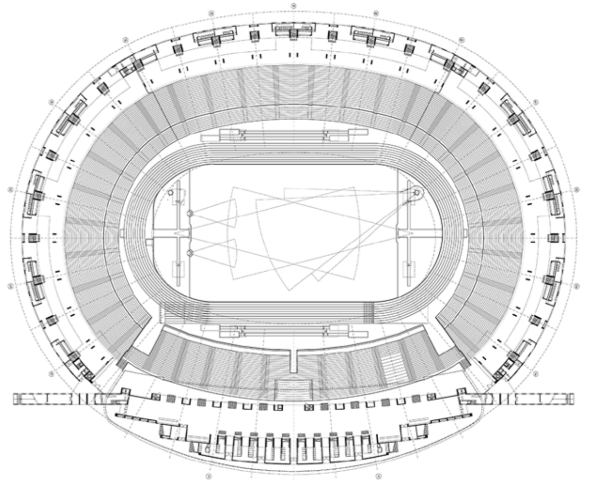
Ground floor
