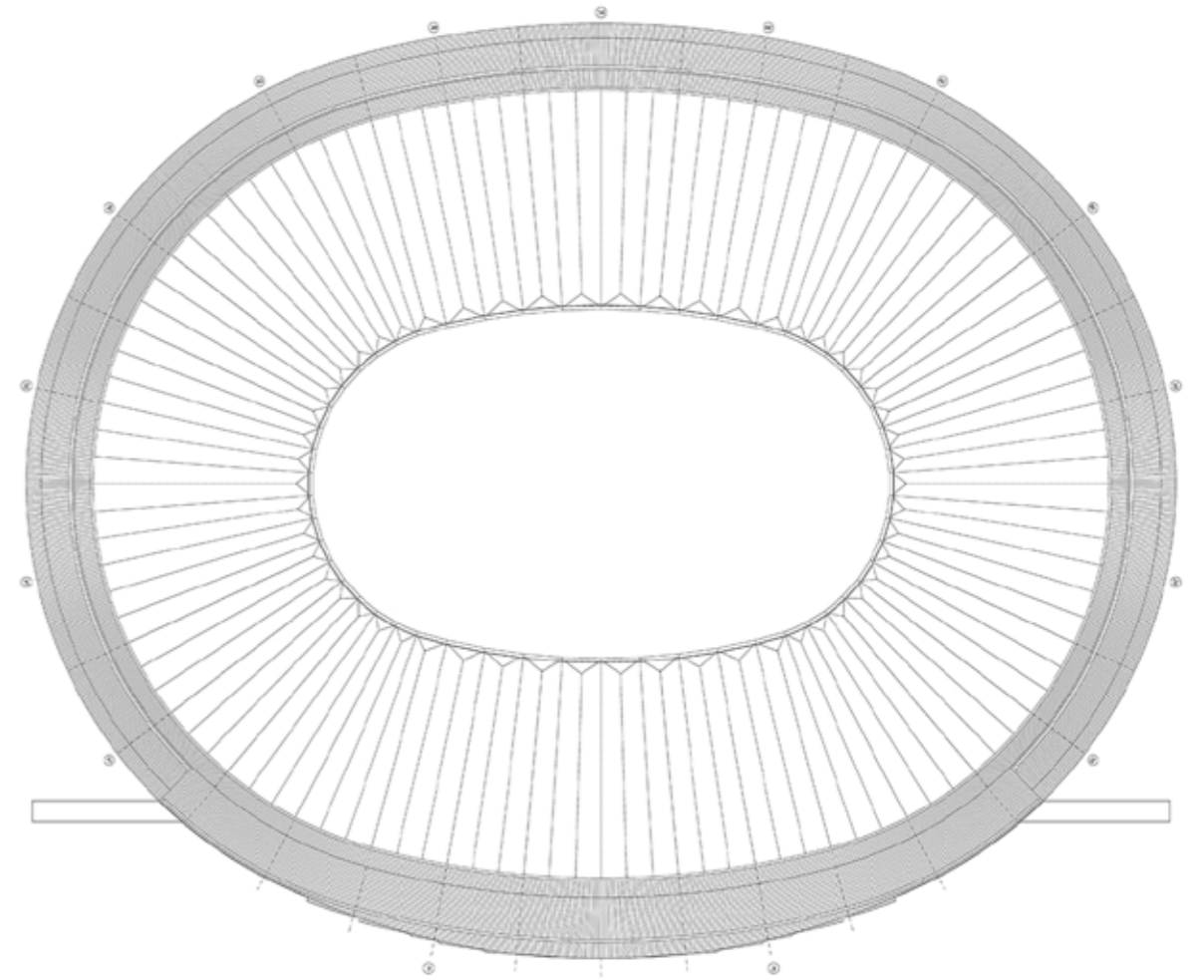
Roof plan
